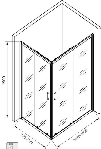
KABINA PRYSZNICOWA MEXO 800x1100x1900
